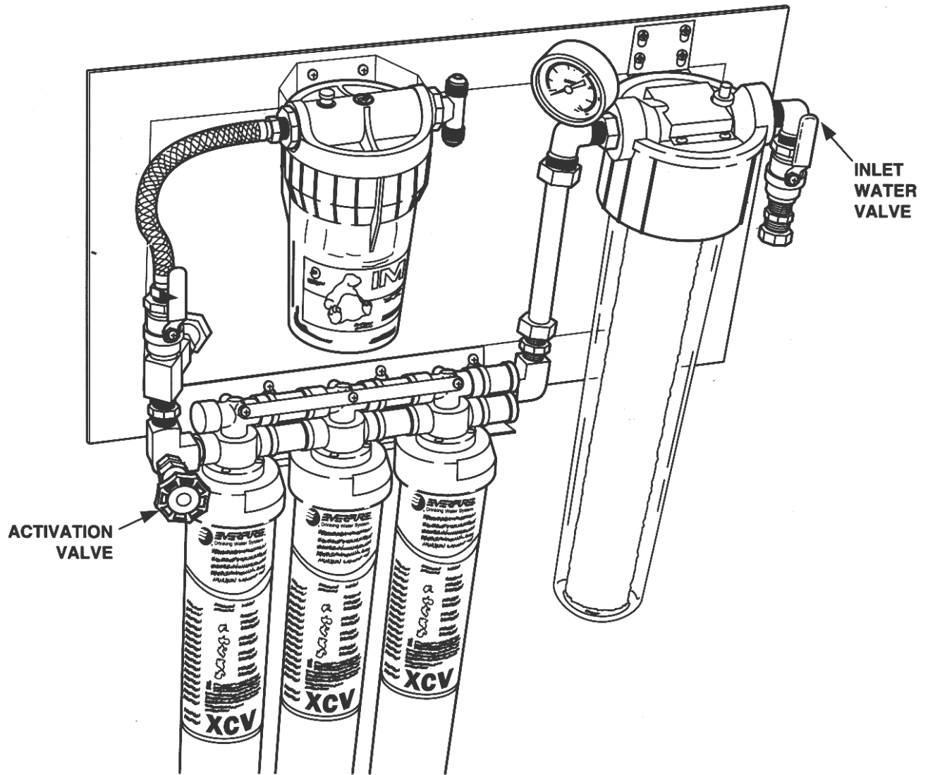
Figure 1—TRI-PACK SYSTEM
