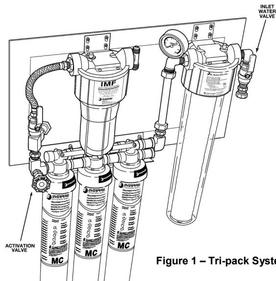
Figure 1 – Quad System
